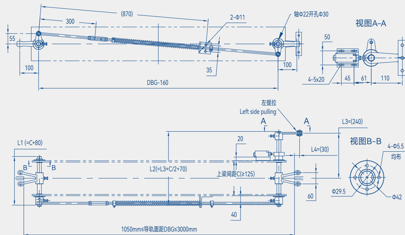
Overall Dimension
