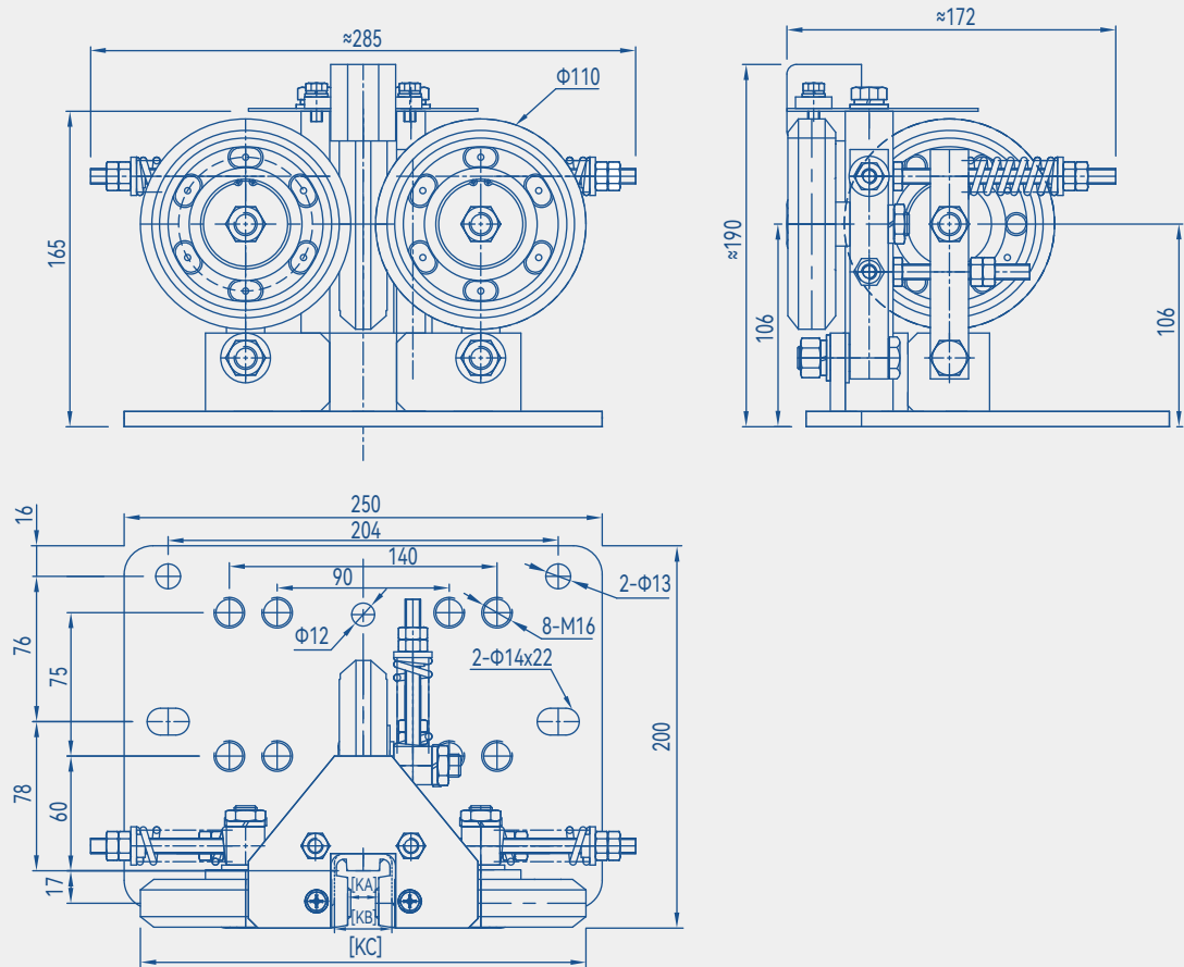
Overall Dimension
