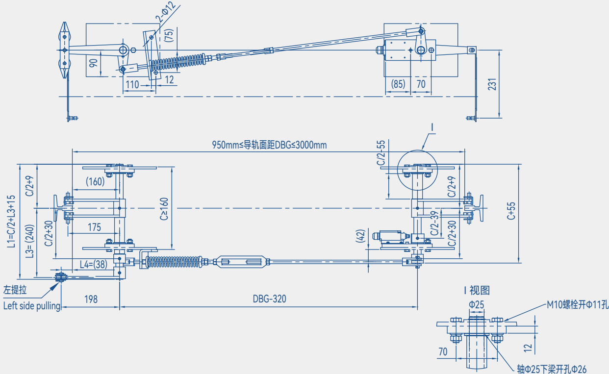
Overall Dimension
