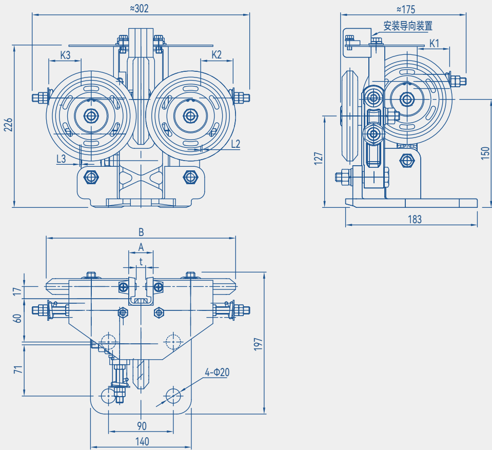
Overall Dimension
