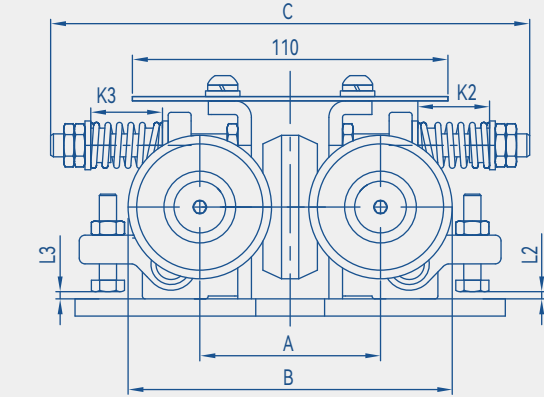
Overall Dimension
