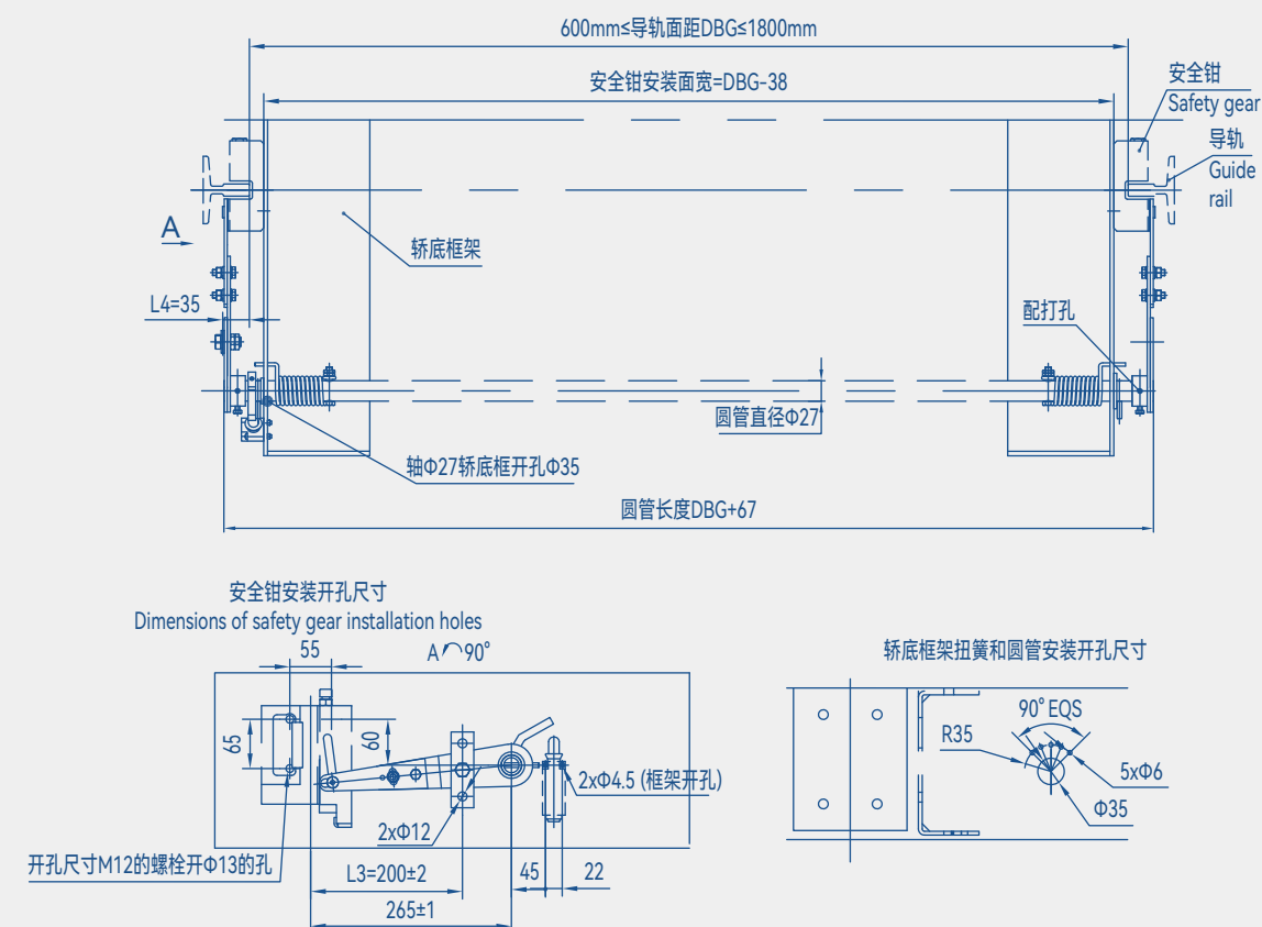
Overall Dimension
