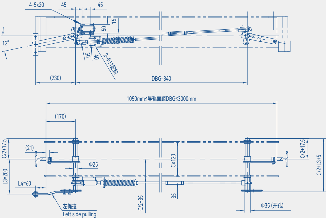
Overall Dimension
