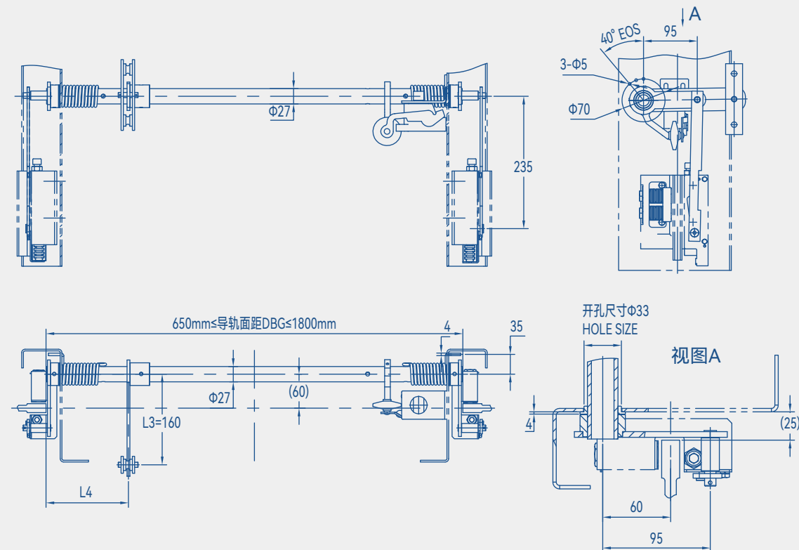
Overall Dimension
