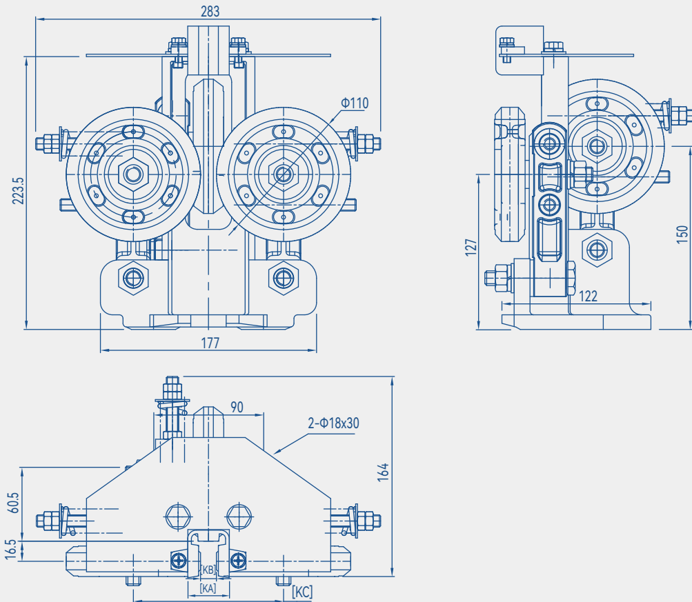
Overall Dimension
