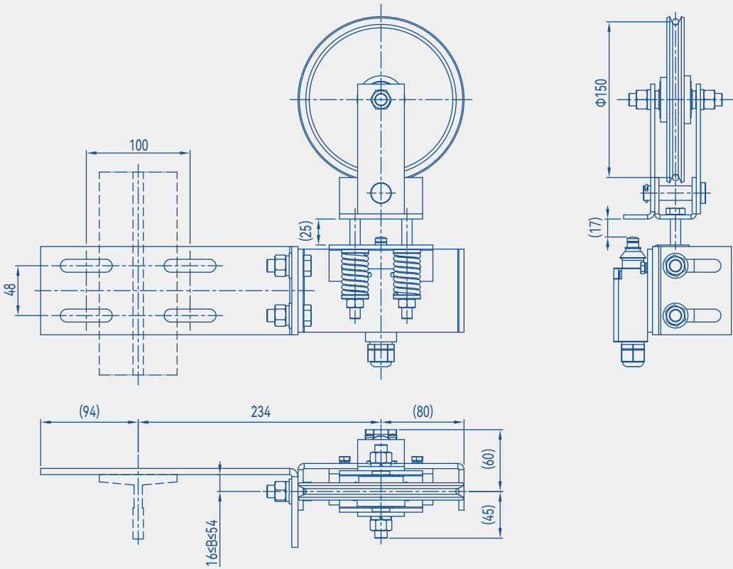
Overall Dimension
