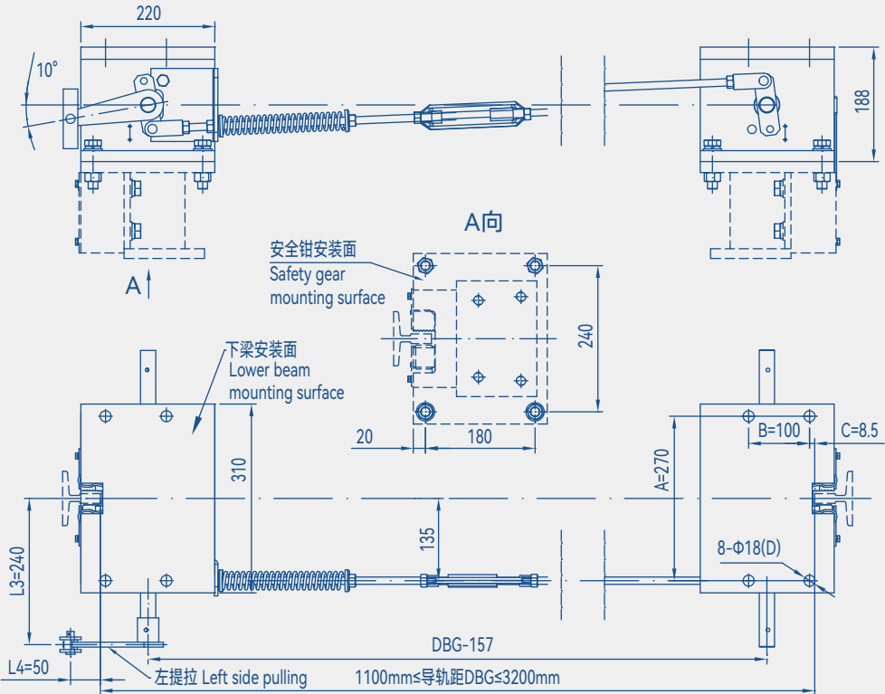
Overall Dimension
