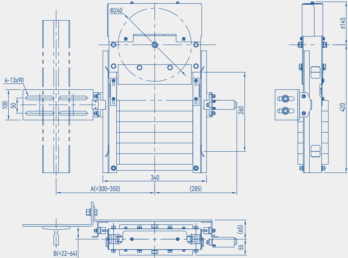
Overall Dimension
